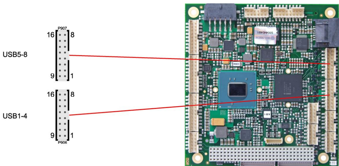
Pinout USB 1-4:
